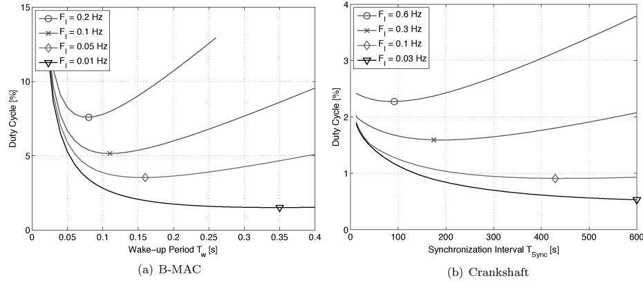
Fig. 8. Optimization of MAC parameters with respect to data load ( F_l ). The markers indicate the optimal operating points of the protocols for different data loads.
