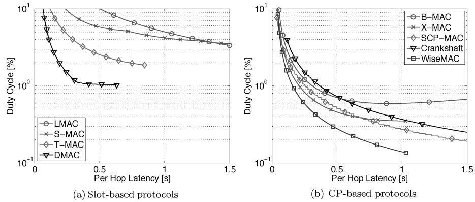
Fig. 10. Energy-latency trade-off (after optimization of MAC parameters).
